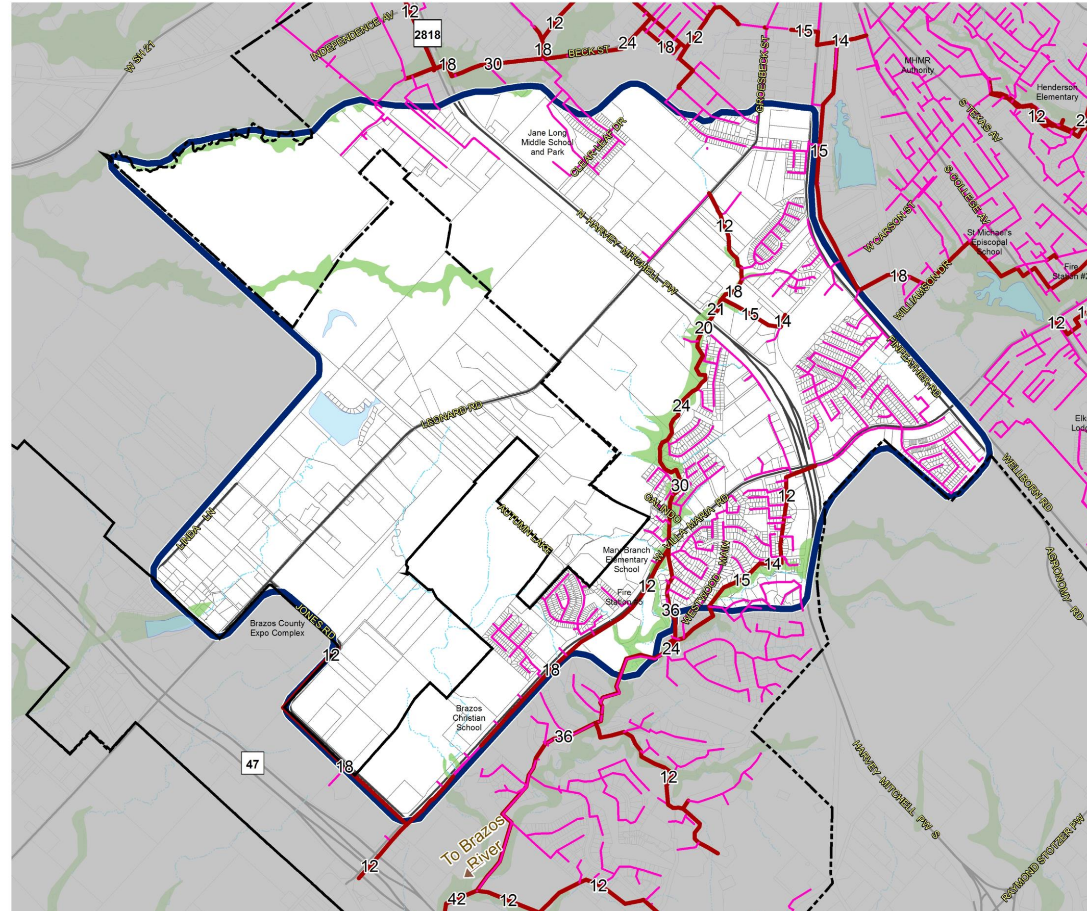
Figure 24: Study Area Wastewater System
