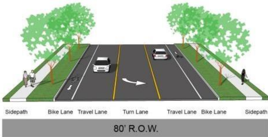
Figure 13: Major Collector
