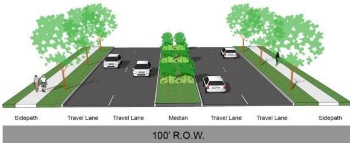
Figure 12: Minor Arterial
